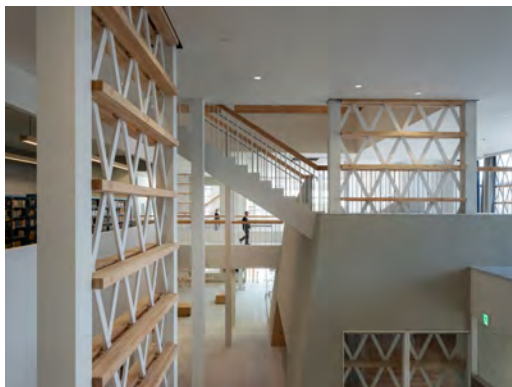
土佐市複合文化施設 Tosa City Cultural Complex Civic hall, library, community center, etc 2019
